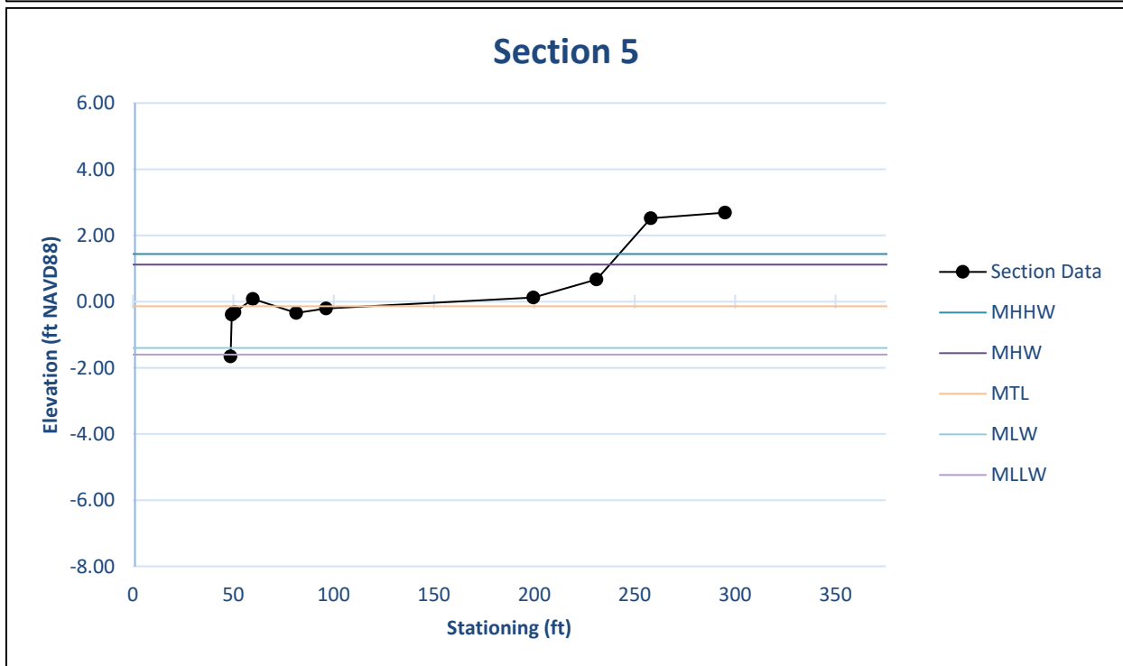
Figure 12: Section 4 and 5 surveyed reflect the elevation in the marsh and edge of farm fields along the southern and eastern edges of the marsh respectively.
