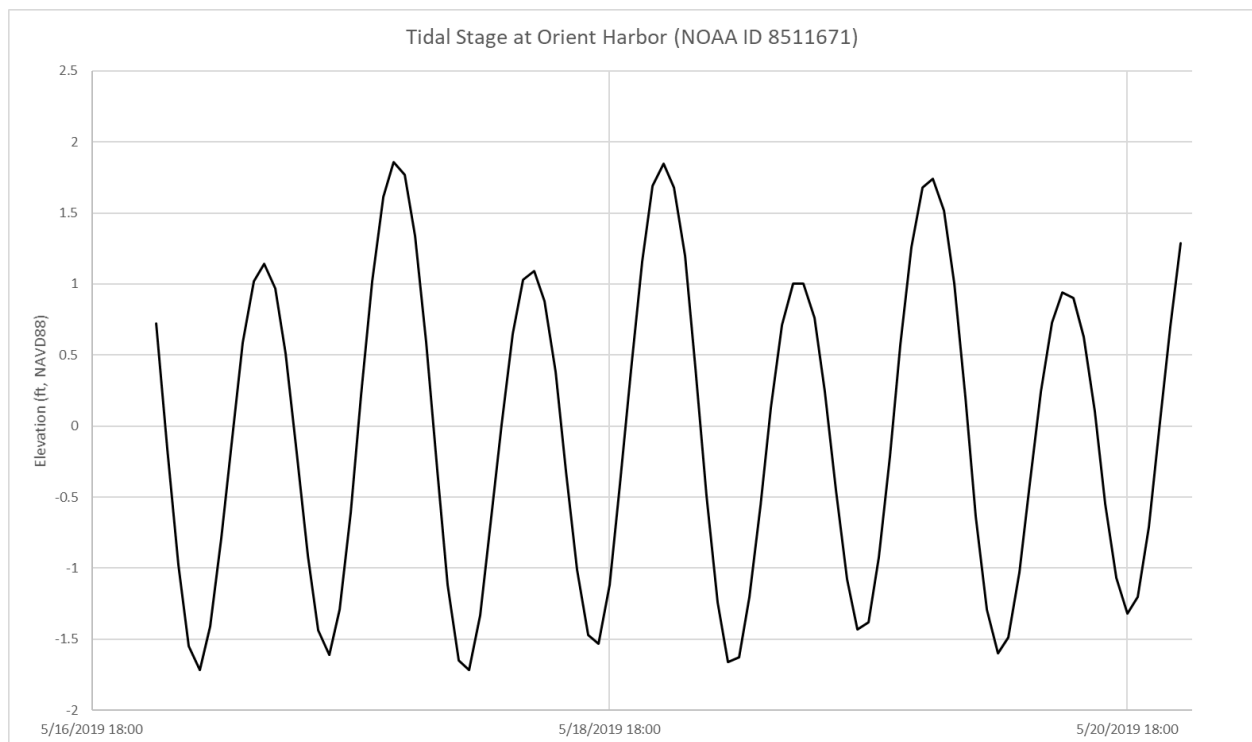
Figure 1. Input tidal hydrograph used for the culvert analysis.
