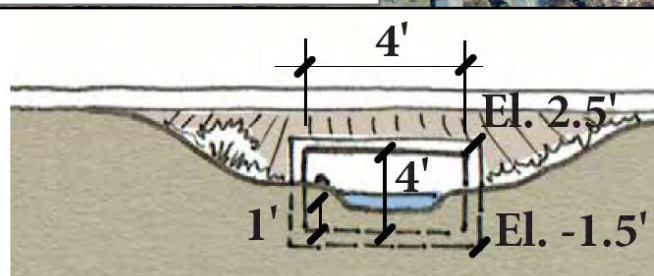
Example photo and sketch of a box culvert with natural bed substrate (courtesy of Resilient Crossings Handbook)
