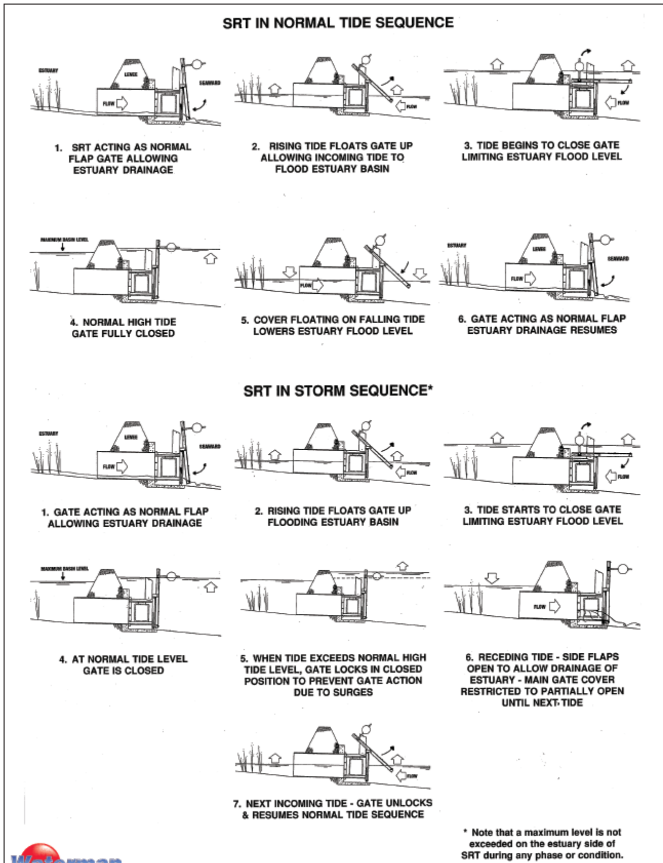
Figure 21: Typical operation of a self-regulating tide gate (Waterman Industries).
