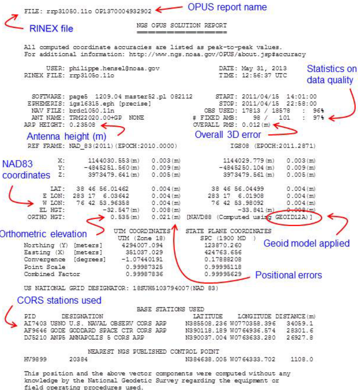
Figure 6.16. Sample OPUS report for a static GPS eight hour, 57 minute observation.
