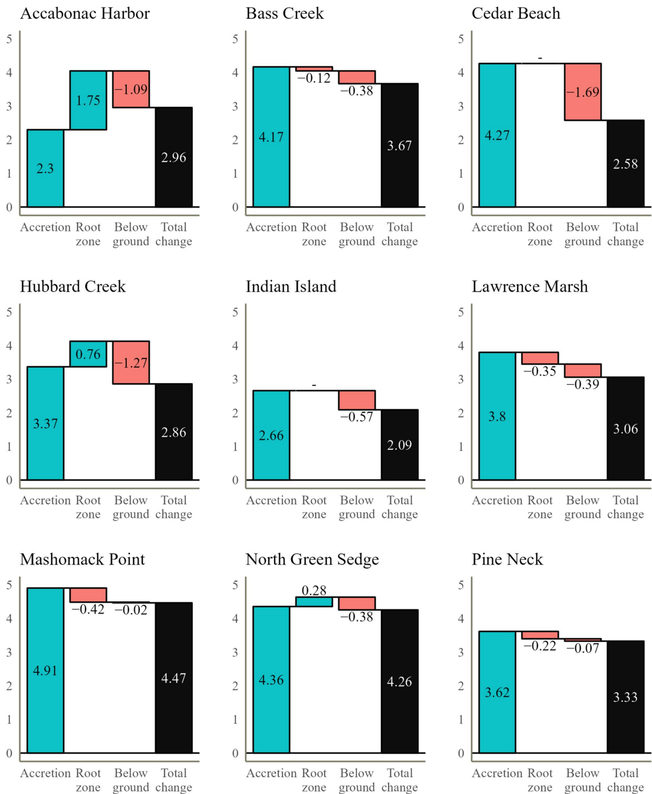
Fig. 8 Waterfall plot displaying the contributions (positive values in blue), reductions (negative values in red), and resulting overall change observed (in black) over the course of this sampling effort. Cedar Beach and Indian Island marshes do not have shallow RSETs installed. These plots are read from left to right. For example, at Accabonac Harbor, the average surface accretion above the marker
